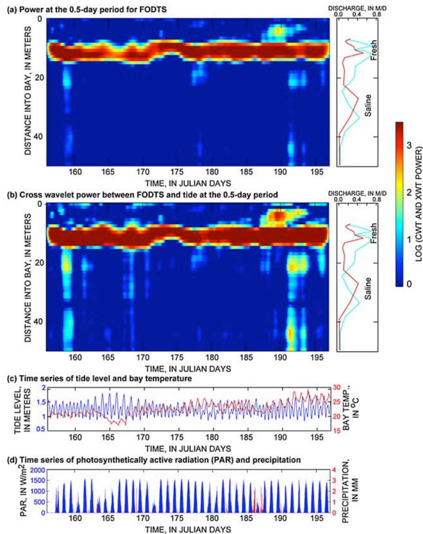
Figure 3. (a) Power at the semi-diurnal period for the FODTS as a function of location and time with measured discharge rates in meters per day (m/d) [after Michael et al. , 2005]; (b) XWT power between FODTS and tide at the semi-diurnal period as a function of location and time with measured discharge rates [after Michael et al. , 2005]; (c) time series of tide level (blue) and surface-water temperature (red); and (d) time series of photosynthetically active radiation (PAR) (blue) and precipitation (red).
